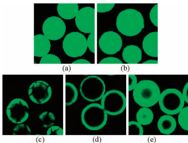
Figure 1. Cross-sectioned confocal microscope images of FITC-coupled resins: (a) TentaGel resin (0.3 mmol NH 2 /g); (b) AM-PS resin (0.3 mmol NH 2 /g); (c) CS resin I (0.5–2 equiv of CNC used, 0.03–0.1 mmol NH 2 /g); (d) CS resin II (3–5 equiv of CNC used, 0.2–0.4 mmol NH 2 /g); (e) CS resin III (7–10 equiv of CNC used, 0.5–0.7 mmol NH 2 /g).
