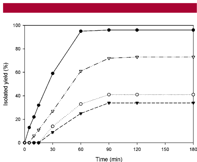
Figure 3. Kinetic profiles of photolytic cleavage on each resin: (●) CS resin, (▽) TentaGel resin, (○) LL PS resin, (▼) HL PS resin.
