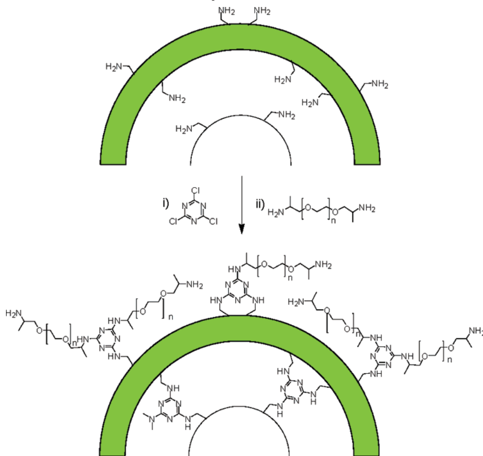
Scheme 1. Preparation of Core–Shell Resins
