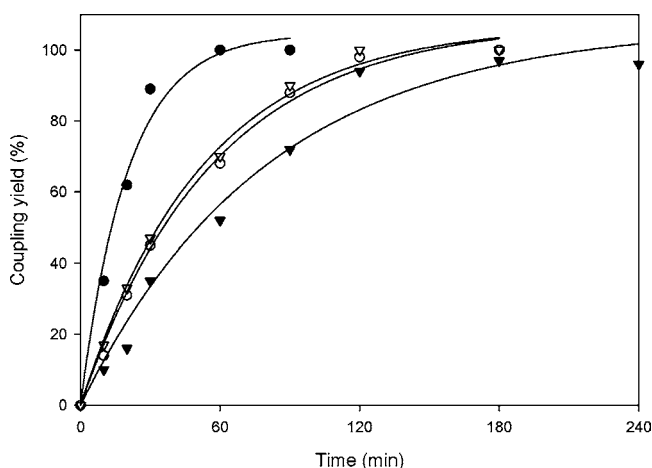
Figure 2. Initial loading time of Fmoc-Leu on the resins: (●) CS resin, (▽) TentaGel resin, (○) LL PS resin, (▼) HL PS resin.
